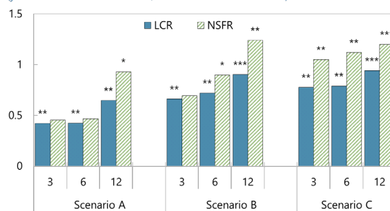
Sensitivity of Remaining CBC to Liquidity Ratios
