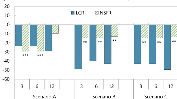
Median Comparison of LCR and NSFR by Scenario
