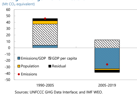
Portugal: Change in GHG Emissions
