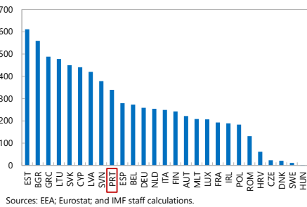
Carbon Intensity: GHG emission per unit of GDP, 2019
