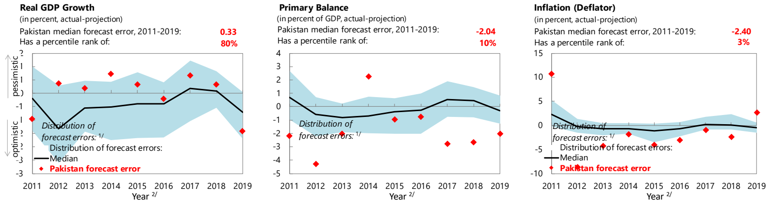
Figure 2. Pakistan: Public DSA – Realism of Baseline Assumptions
