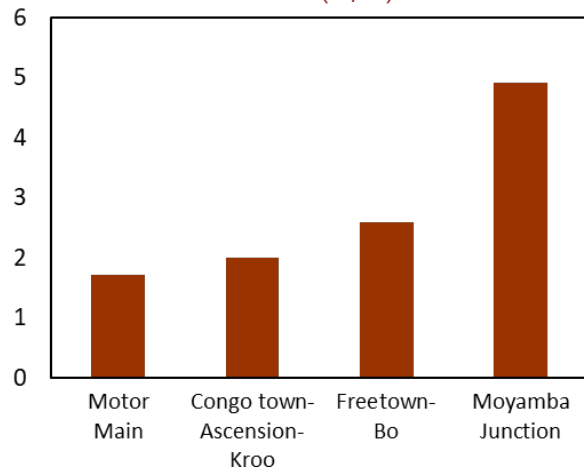
Figure 17. Maximum Shocks from Roads to Vehicles (m/s 2 )
