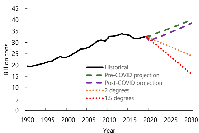
Figure 1. Global Fossil Fuel CO 2 Emissions Trends
